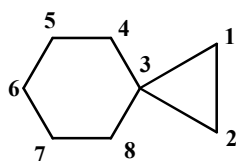
spiro[2,5]octane
