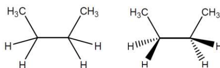
Perspective
