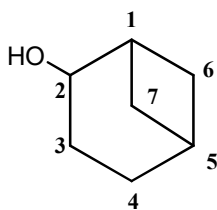
bicyclo[3,1,1]heptan-2-ol
