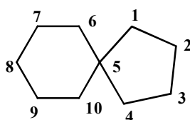
spiro[4,5]decane
